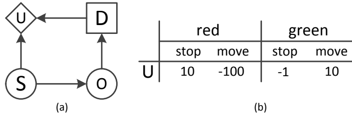
Fig. 3. (a) The influence diagram for decision making based on information observed from a signal. (b) The utility table for U(D, S) .
