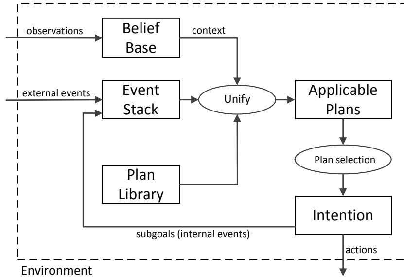
Fig. 1. The reasoning cycle of an AgentSpeak agent
