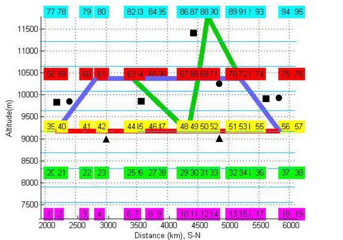
Fig. 10. Vertical track variation through wind map 1 for wind optimal (blue ●), constant fuel burn wind optimal (green ■) and shortest distance (red ▲) routes between Waypoints 40 and 56. Fuel savings are 4.31% for varying fuel burn model and 2.29% for constant fuel burn model.
