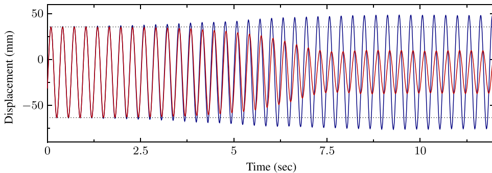
Fig. 5. Two separate time-series measurements in taken open-loop conditions starting from the same unstable periodic orbit. The measurements were synchronised using the periodic forcing as a reference signal. Noise in the experiment randomly perturbs the trajectory from the unstable periodic orbit to either the stable high-amplitude orbit (blue) or the stable low-amplitude orbit (red). This shows that the stable manifold of the unstable periodic orbit acts as a separatrix between the basins of attraction of the high- and low-amplitude orbits. (For interpretation of the references to color in this figure caption, the reader is referred to the web version of this paper.)
