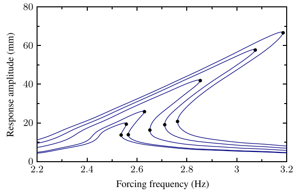
Fig. 4. A series of frequency response curves extracted from the data shown in Fig. 3 using Gaussian process regression. The forcing amplitudes of the base motion are 1.9, 2, 2.5, 3 and 3.5 mm respectively. Fold points (limit points) which determine the hysteresis region are marked with black dots.
