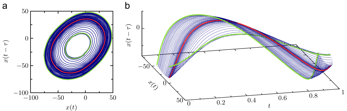
Fig. 9. State-space projections in 2D and 3D of the data shown in Fig. 5 using time-delay coordinates. The red curve represents the unstable periodic orbit and the two green curves represent the stable high- and low-amplitude periodic orbits. The blue curves show the transient dynamics between the unstable orbits and the stable orbits. The two different stable orbits are reached with approximately equal probability. The time coordinate in panel (b) is normalised such that a period of forcing takes one time unit. (For interpretation of the references to color in this figure caption, the reader is referred to the web version of this paper.)
