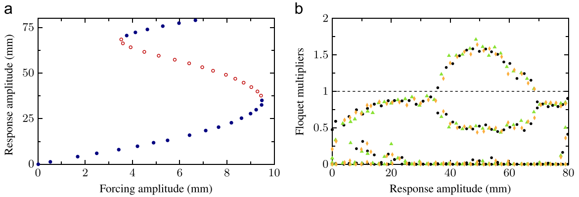
Fig. 8. Panel (a) shows a single continuation with the response amplitude plotted against the forcing amplitude for a fixed forcing frequency of 3.2 Hz. Stable periodic orbits are shown by solid blue dots and unstable orbits are shown by red circles. The maximum displacement of the experiment is limited to \pm 80 mm. Panel (b) shows the absolute value of the estimated Floquet multipliers plotted against the response amplitude for three separate continuation runs (each shown with a different symbol). It can be seen that most of the stable periodic orbits have complex conjugate Floquet multipliers which then become real close to the saddle-node bifurcations; between the two saddle-node bifurcations, one of these Floquet multipliers lies outside the unit circle while the other lies inside the unit circle. (For interpretation of the references to color in this figure caption, the reader is referred to the web version of this paper.)
