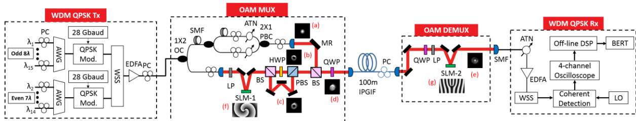
Fig. 1. Experiment setup of the transmission system. Insets (a)-(c): mode profiles of \text{OAM}_0 , \text{OAM}_{+2} and \text{OAM}_{-2} ; (d) profile of the four multiplexed modes; (e) de-multiplexed mode \text{OAM}_{+2R} ; (f)-(g): phase patterns for ‘perfect’ vortex generation and de-multiplexing.
