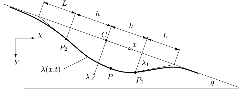
Figure 3: Tyre deformation according to the stretched string tyre model. The turning angle \theta is between the direction of motion X and the intersection of the ground and the wheel plane
