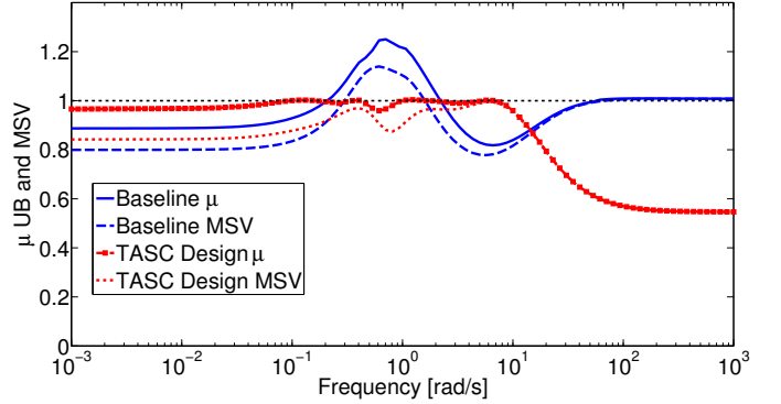
Fig. 5. Lateral Plant RP with two different controllers
