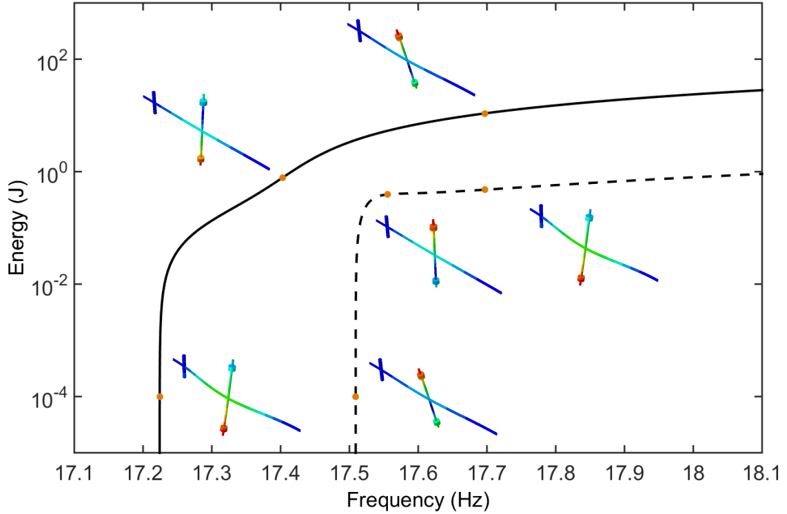
Figure 3: Frequency-energy plot of the nonlinear normal modes of the clamped-clamped cross beam structure ROM. (—) First NNM; (---) second NNM. Mode shapes are inset.
