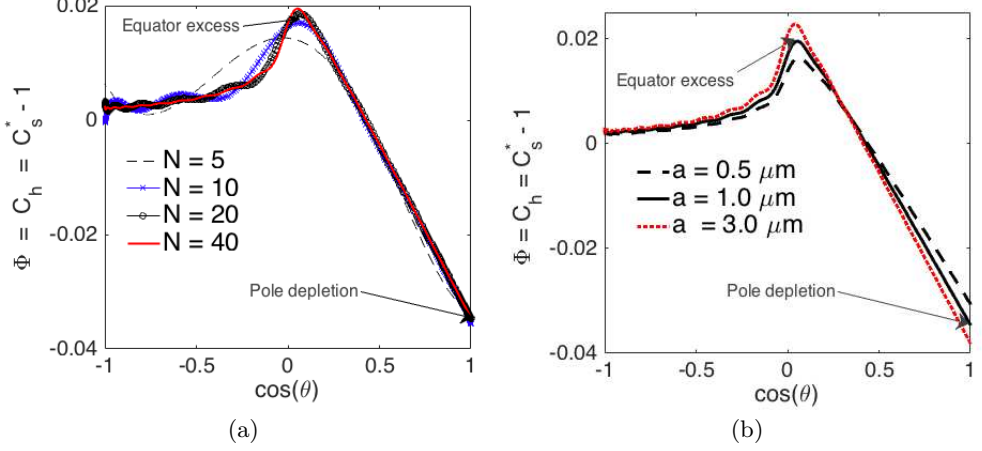
FIGURE 5. (a) The deviations of the surface electric potential, \Phi(1, \theta) , and ionic concentrations, C_h(1, \theta) , C_s^*(1, \theta) - 1 , from the uniform background values (for swimmer size a = 1.00 \mu\text{m} ). We show the convergence of the solution as the number N of the Legendre modes in eqn. (3.34) are increased, i.e. \mathbf{A} = \{A_0, \dots, A_{N-1}, A_N\} . (b) The deviations of the surface potential and ionic concentration as a function of swimmer size a (truncating at N = 40 ).
