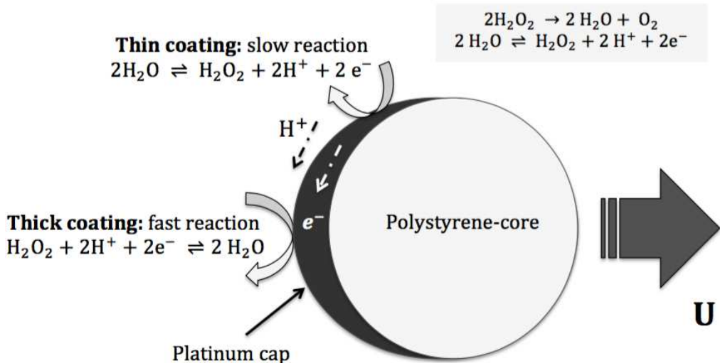
FIGURE 1. Cross-section of a schematic swimmer showing the variation of the thickness of the Pt-coating, the directions of the currents and swimming direction.
