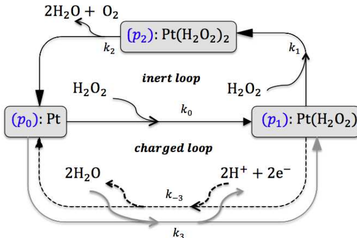
FIGURE 9. ( Reaction scheme 1 ): Schematic complexation kinetics of the Platinum catalyst with free (0'th state) Pt occupied with probability density p_0 ; first complex state \text{Pt}(\text{H}_2\text{O}_2) occupied with probability density p_1 , and the second complex state \text{Pt}(\text{H}_2\text{O}_2)_2 occupied with probability density p_2 .
