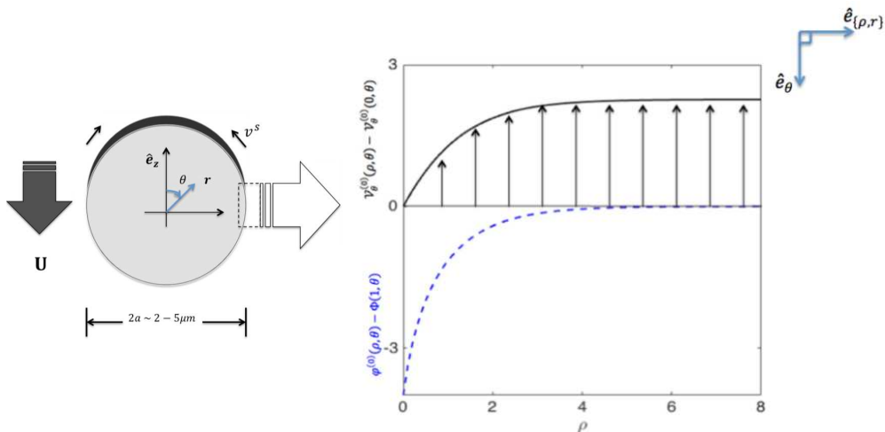
FIGURE 3. Profiles of flow and electric field within the (inner) Debye layer with C_s^* = \partial C_s^* / \partial \theta = \partial \Phi / \partial \theta = 1 (see Appendix B).
