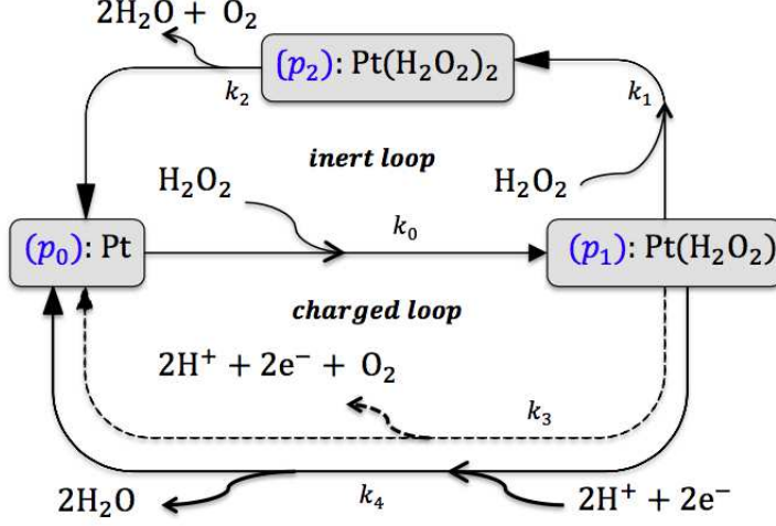
FIGURE 10. ( Reaction scheme 2 ): Schematic complexation kinetics of the Platinum catalyst with free (0'th state) Pt occupied with probability density p_0 ; first complex state \text{Pt}(\text{H}_2\text{O}_2) occupied with probability density p_1 , and the second complex state \text{Pt}(\text{H}_2\text{O}_2)_2 occupied with probability density p_2 .
