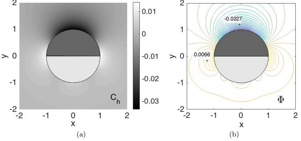
FIGURE 4. (a) Proton concentration deviation from the uniform background profile and (b) associated electric potential difference contours (both plots with pH = 5.5 for 10% H 2 O 2 without salt and the system parameters in table (1)). The equipotential contours 0.0066 and -0.0227 (in units of the thermal voltage ( k_B T/e ) \approx 25 mVolts) are shown to indicate the electric pole-equator polarity. In both figures, the upper (dark) hemisphere is the Platinum cap.
