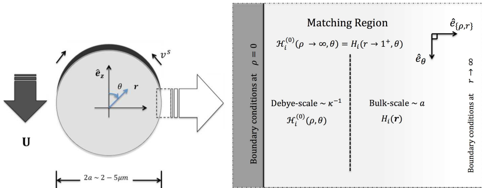
FIGURE 2. Schematic Platinum-Polystyrene swimmer and the domain decomposition of the phoretic problem.
