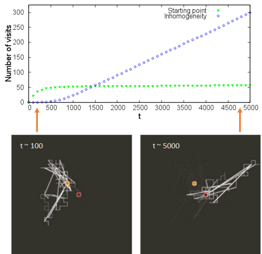
FIG. 1. (Color online) Average total number of visits to the starting site \mathbf{x}_0 = (-5, 5) (green triangles) and to the inhomogeneity (blue diamonds) as function of time, for a 2d walker with q = 0.2 ( \gamma = 0.9 ). At early times, the walker slowly diffuses around \mathbf{x}_0 (orange-light disk in the insets). After the inhomogeneity (red-dark disk) has been found, it becomes steadily revisited, indicating spatial learning and localization.
