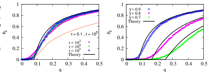
FIG. 3. (Color online) Phase transition in 1d for Lévy flights with \mu = 1/2 . Left: The thick (black) solid lines are given by Eq. (5) for the t \rightarrow \infty limit, and the symbols by simulations up to different times t ( \gamma = 0.9 ). The parameter \tau is explained in the text, end of p. 4. Right: P_0 for \gamma = 0.9, 0.8 and 0.7 , where theory predicts q_c \approx 0.0803, 0.1642 and 0.2519 , respectively ( t = 10^5 in simulations).
