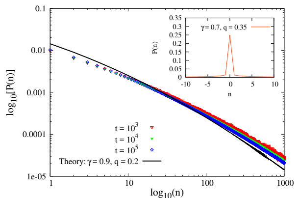
FIG. 5. Asymptotic probability of presence in 1d for Lévy flights with \mu = 1/2 . The solid line is the inverse Fourier transform of Eq. (4) and symbols represents simulations.
