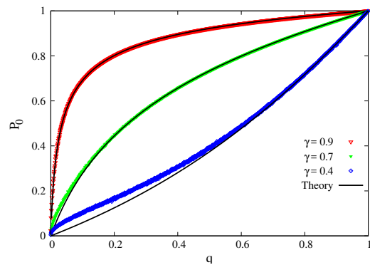
FIG. 2. (Color online) P_0 as a function of q in 1d with n.n. hopping. Solid lines are given by Eq. (8) and symbols by Monte Carlo simulations of the rules (a)-(b) (at t = 10^5 ).
