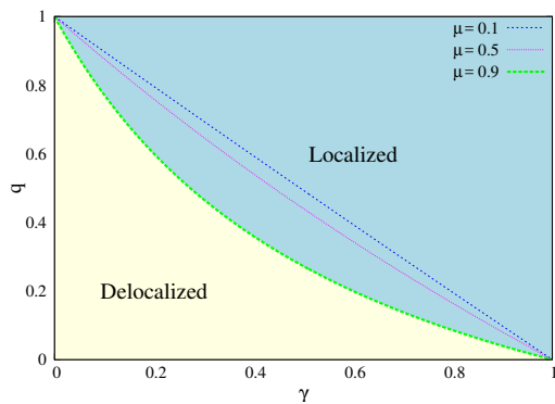
FIG. 4. (Color online) Phase diagram in 1d for various Lévy indexes.
