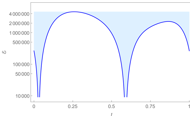
Figure 2: The domain of definition \bar{\Lambda} of the scattering map S_{\Gamma} , in physical variables (\mathcal{E}, t) . The dark blue curve is the graph of \left(\frac{|a \frac{db}{dt} - b \frac{da}{dt}|}{|\delta|} \phi(t)\right)^2 , with \phi(t) given by (50). The shaded region is the domain \bar{\Lambda} . Here a(t) = 5 + \sin(2\pi t) , b(t) = 2 - \cos(2\pi t) , \delta = 0.05 .
