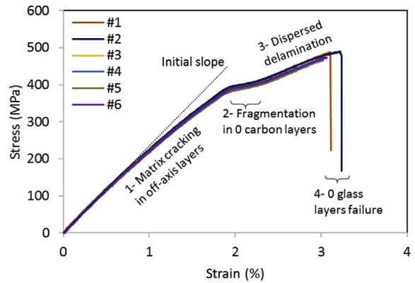
Fig. 8. Tensile stress-strain curves of the orientation-dispersed hybrid quasi-isotropic laminate [45_C/90_C/-45_C/0_C/0_C/45_C/90_C/-45_C]_S .
