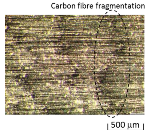
Fig. 11. Optical microscopy image from the top view of the 0 carbon layer showing the fragments.
