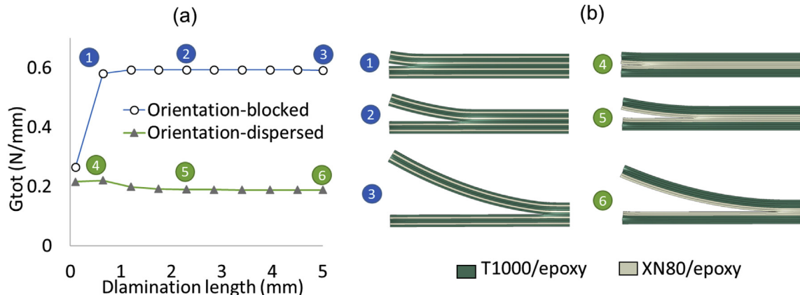
Fig. 4. (a) Total energy release rate ( G_{tot} ) of the orientation-blocked and orientation-dispersed laminates with different delamination lengths at the most susceptible interface.
