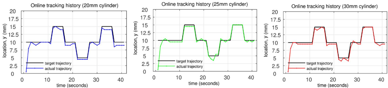
Fig. 11. Online tracking of multiple objects (20 mm, 25 mm and 30 mm diameter cylinders). Target trajectories are pre-set locations. The actual trajectory shows the movements of the robotic finger during manipulation.
