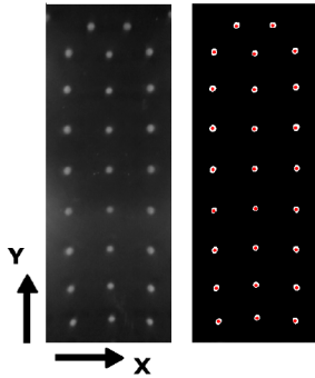
Fig. 4. Images recorded by the TacThumb. The left panel shows the image captured. The right panel shows the image after pre-processing - red dots represent the pin centers identified by the pin detection algorithm.
