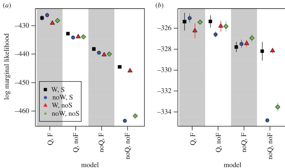
Figure 2. Model selection results. We show the marginal likelihood for each model averaged over five numerical model fitting replicates for the data in the absence (a) and presence (b) of the M treatment. Error bars show 1 s.d. and are often smaller than the symbol size. Grey bars serve to separate ‘blocks’ of models (see main text). We construct models by accounting for different aspects of the virtual environment that are captured by two time-independent model components (W, exit width; S, exit route length) and two time-dependent model components (Q, queue length; F, queue speed). For example, the first model on the left-hand side in (a) (Q, F, W, S), includes all four model components, and the model to its right (Q, F, noW, S) includes all model components, apart from W.
