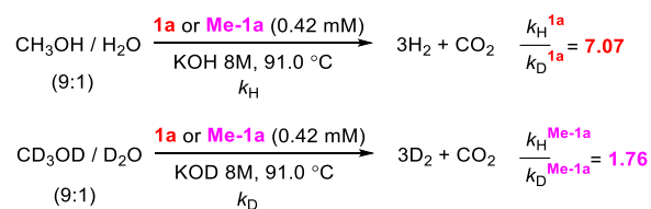
Scheme 4. KIE measurements for catalyst 1a and Me-1a .
