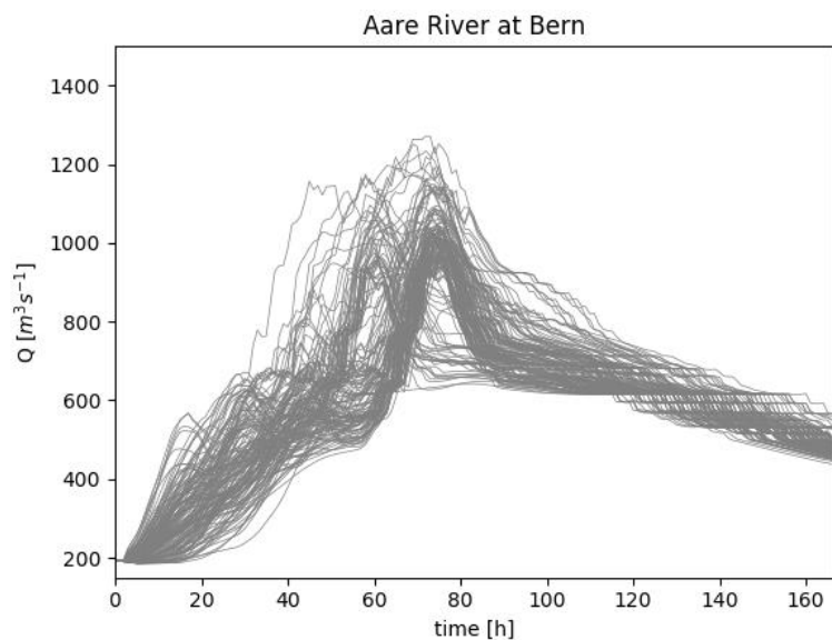
Figure 3: Hydrographs at the outlet of the Aare River basin in Bern resulting from the coupled hydrologic-hydrodynamic modelling of the 150 PMP scenarios.
