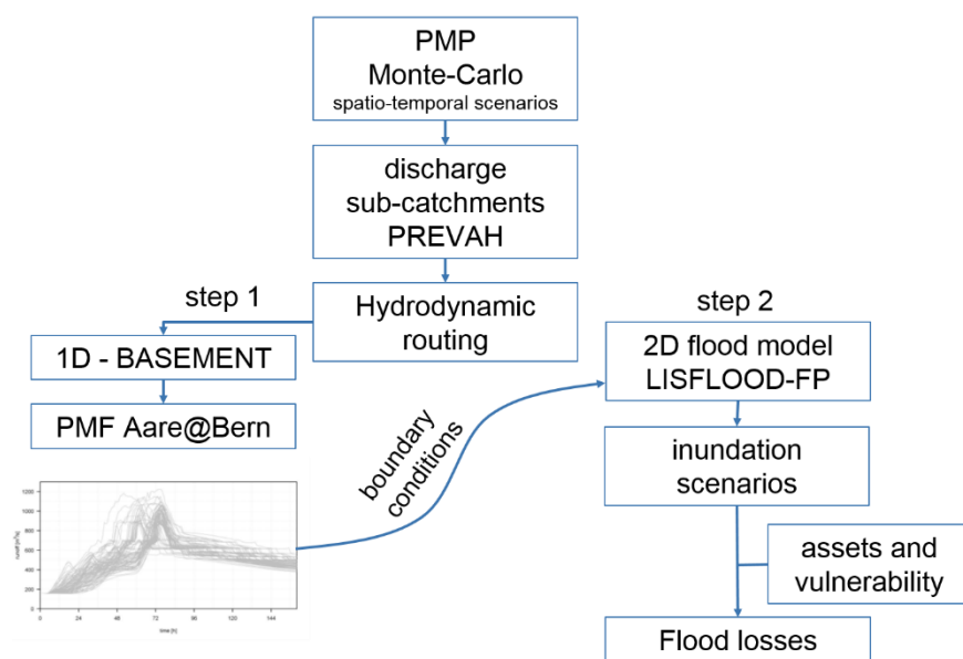
10 Figure 1: Schematic of the nesting approach. The 2D flood inundation models and the loss models are nested in a 1D routing model.
