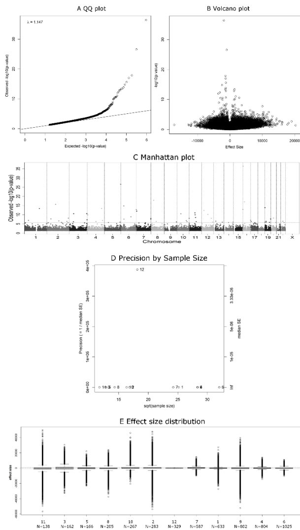
Figure 1. Diagnostic plots showing cohort-specific (A-C) and between-cohort QC characteristics (D-E) produced by QCEWAS.
