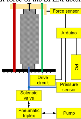
FIGURE 5. Schematic diagram of the SFLM output force testing platform.
