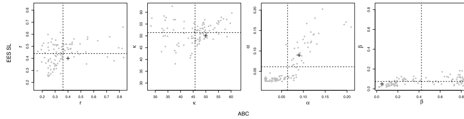
FIG 2. MLE estimates obtained using EES SL versus MAP estimates produced by ABC, under model (1). The dashed lines and the black crosses indicate, respectively, the mean estimates under each method and the true parameter values.
