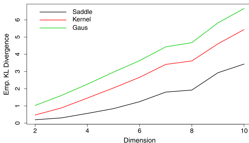
FIG 5. Empirical Kullback-Leibler divergence between the three density estimators and the true density, as the number of dimensions increases.
