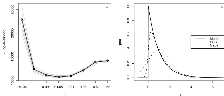
FIG 3. Shifted exponential model. a: Curves from 10-fold cross-validation, the black line is their average. b: True \text{Exp}(\beta) density (black), EES (dashed) and normal (dotted) approximation.
