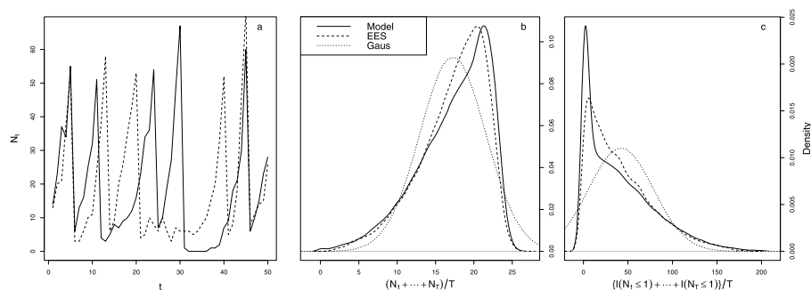
FIG 1. a : First 50 steps of two sample paths, simulated from model (1). b and c : Marginal distributions of the population mean and of the number of periods t during which N_t \leq 1 , when T = 250 . Both distributions are highly skewed, and the EES density achieves a much better fit than a Gaussian approximation.
