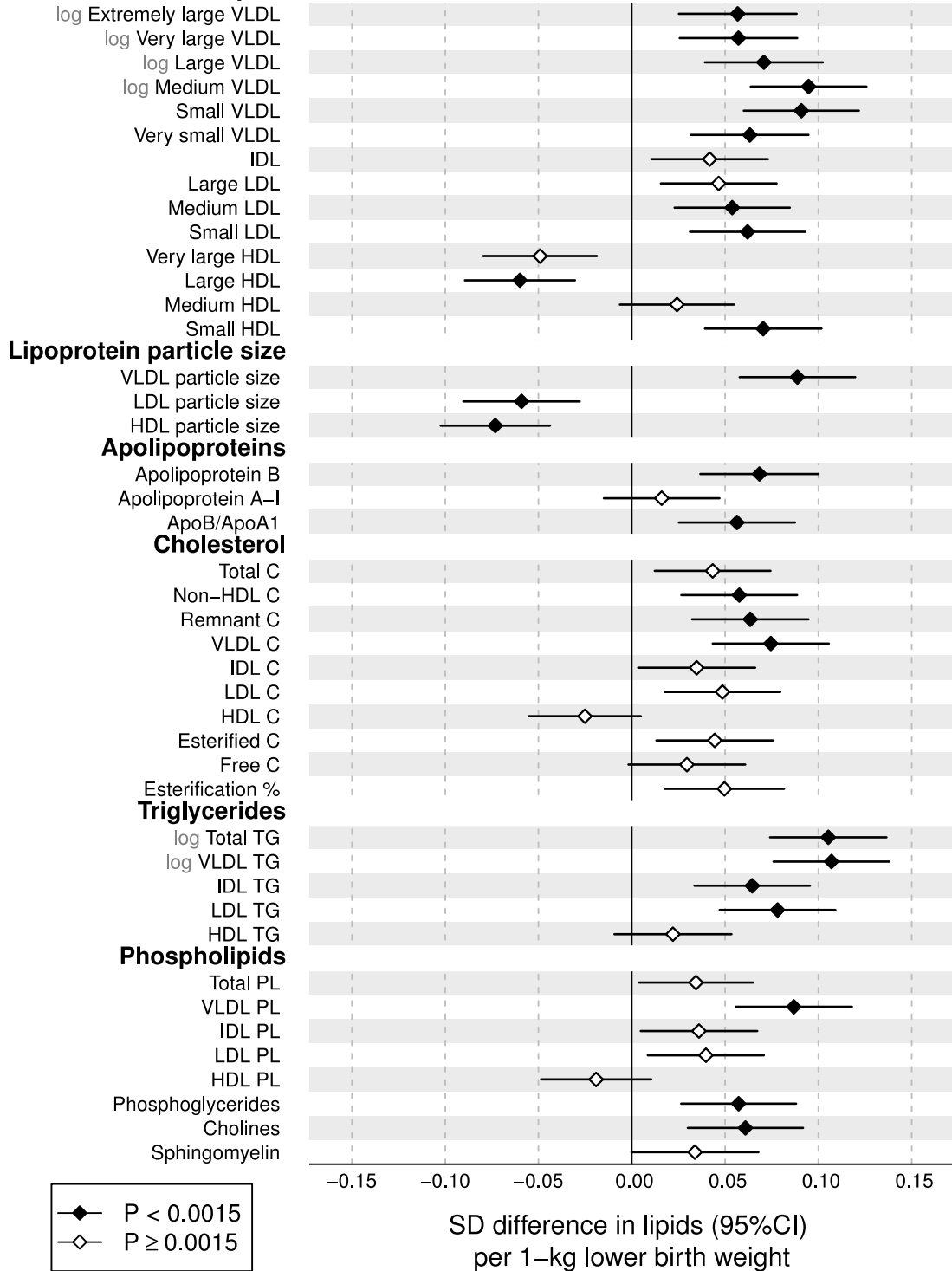
Figure 1. Birth weight associations with adult concentrations of lipoprotein lipids. The associations were adjusted for sex, gestational age, and age at blood sampling, and meta-analysed for 18 288 individuals from 7 cohorts. Association magnitudes are 1-SD lipid concentration per 1-kg lower birth weight. Error bars denote 95% confidence intervals. Filled diamonds indicate P < 0.0015 . Association magnitudes in absolute concentration units and P-values are listed in Table S1 . Results for individual cohorts are shown in Figure S5 .
