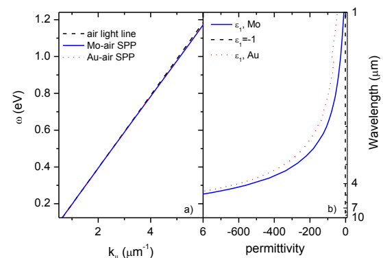
Figure 1 Optical characteristics of gold and molybdenum (a) Analytic dispersion curve of surface plasmon polaritons supported by an air-molybdenum interface (blue line) and
