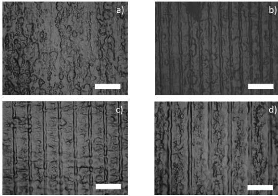
Figure 3. Optical microscope images of the surface of thermally tested Molybdenum samples: a) bare sample and laser-structured samples with periods of: b) 10.5 \mu\text{m} (10P), c) 15.0 \mu\text{m} (15P) and d) 20.0 \mu\text{m} (20P). Objective magnification 50x. Scale bar 25 \mu\text{m} .
