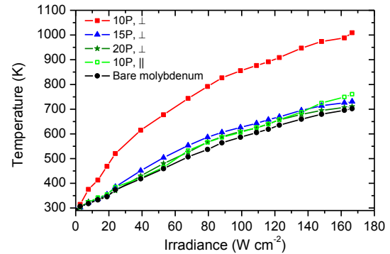
Figure 5 (Colour online). Temperature vs laser power irradiance plots of a bare molybdenum substrate (black circular dots) and three molybdenum gratings with the laser polarization perpendicular to the grating grooves. 15P corresponds to the grating with the period 15 \mu\text{m} (blue triangular dots). 20P corresponds to the grating with period 20 \mu\text{m} (green star dots). 10P corresponds to the grating with a period of 10.5 \mu\text{m} (red full square dots). Also we have included the temperature achieved at different laser power intensities with the polarization of the laser parallel to the gratings grooves for 10P sample (green empty square dots).
