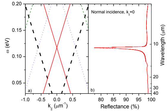
Figure 2 Optical characteristics of a molybdenum grating a) Analytical dispersion curve of surface plasmon polaritons propagating in a molybdenum grating of period 10.5 \mu\text{m} . Black line dashed lines correspond to the light cone lines. Red continuous, blue dotted and green dotted-dashed curves indicated the zero, first and second order light of the molybdenum grating. b) Reflectance associated to the same grating at normal incidence ( k_{\parallel}=0 , see Figure 2.a) showing a minimum at reflectance at 10.6 \mu\text{m} when the surface plasmon polariton mode is excited.
