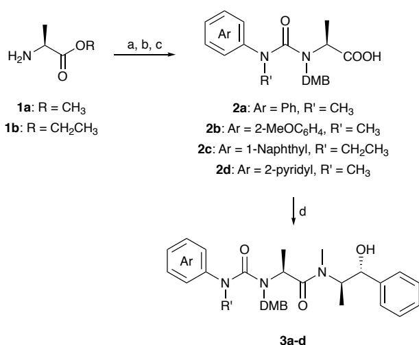
Scheme 1: Reagents and conditions: (a) 2,6-dimethoxybenzaldehyde, NaOAc, NaHB(OAc) 3 , EtOH, rt; (b) ArN(R')COCl, triethylamine, MeCN, reflux; (c) LiOH, THF/H 2 O, 45 ^{\circ}\text{C} ; (d) EDC.HCl, HOBT.H 2 O, ( R,R )-pseudoephedrine, CH 2 Cl 2 , rt. DMB = 2,4-dimethoxybenzyl.
