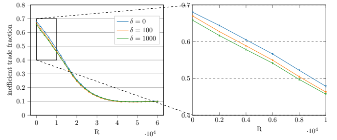
(b) Inefficient trade fraction (inefficiently traded orders / total fulfilled orders). Notice that \delta = 0 (i.e., central CDA) has the highest fraction ( \approx 0.65 ) of inefficient trades when R = 2000 (right, zoomed region).
