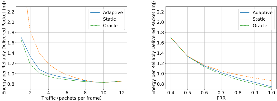
Fig. 4. The energy per reliably delivered packet (Equation 5) of Adaptive Static Scheduling compared against a static schedule that favours reliability and an oracle schedule. Left: depending on traffic rate; right: depending on channel quality.
