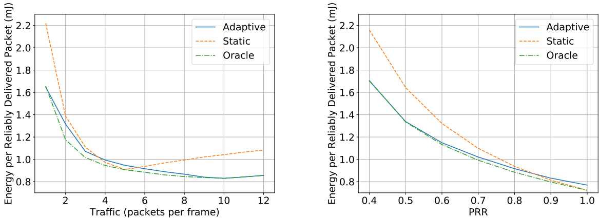
Fig. 5. The energy per reliably delivered packet (Equation 5) of Adaptive Static Scheduling compared against a static schedule that favours energy consumption and an oracle schedule. Left: depending on traffic rate; right: depending on channel quality.
