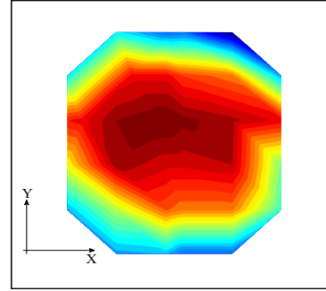
MLA3: 30% Cracked Array, Input Direction: X NN Predicted Displacement Correlation
