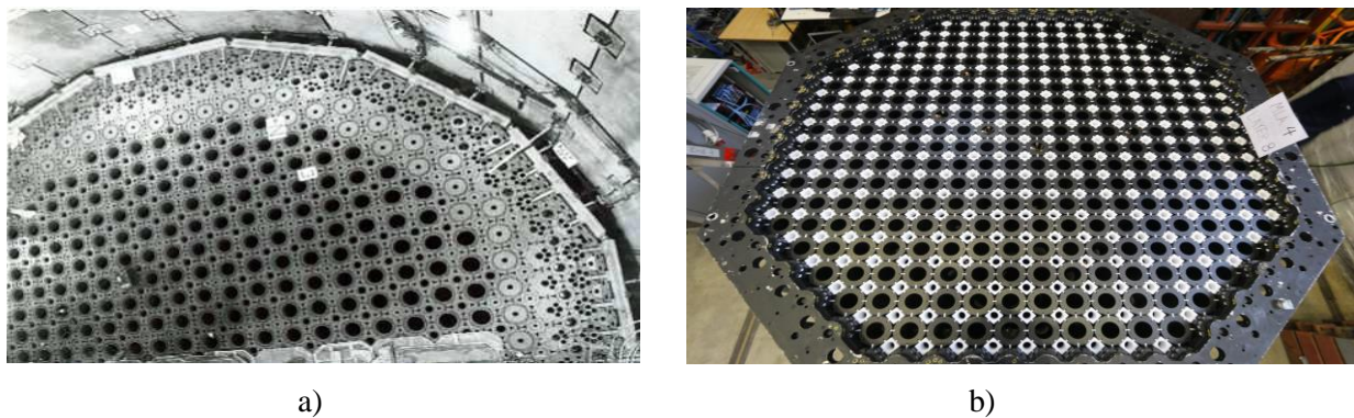
Figure 2 An AGR core (a), courtesy EDF Energy), the MLA rig (b), view from above.
