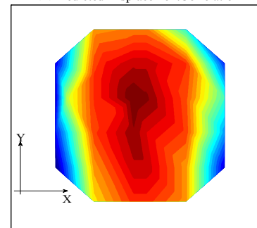
MLA3: 30% Cracked Array, Input Direction: Y NN Predicted Displacement Correlation
