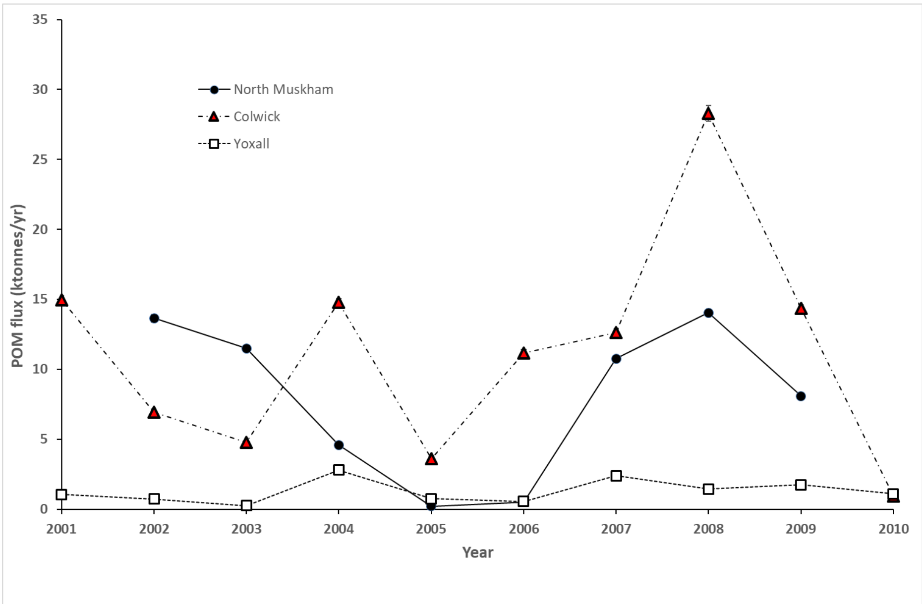
Figure 3. The POM flux from the three monitored sites over the last decade for which POM concentration was available. The error bars are \pm 2\% based on the precision predicted for Equation (i). The values were not bias-corrected.
