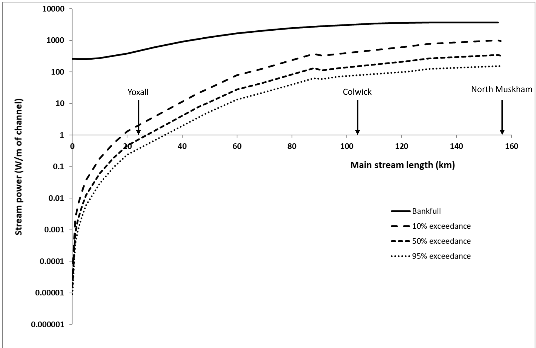
Figure 4. The longitudinal stream power profile for the main channel of the River Trent for a range of flows with the position of monitoring Sites marked.
