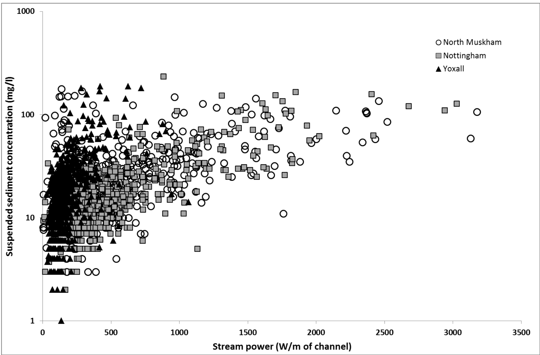
Figure 6. Comparison of the suspended sediment rating curves in terms of stream power for the three stations on the main channel of the River Trent as shown in Figure 2.
