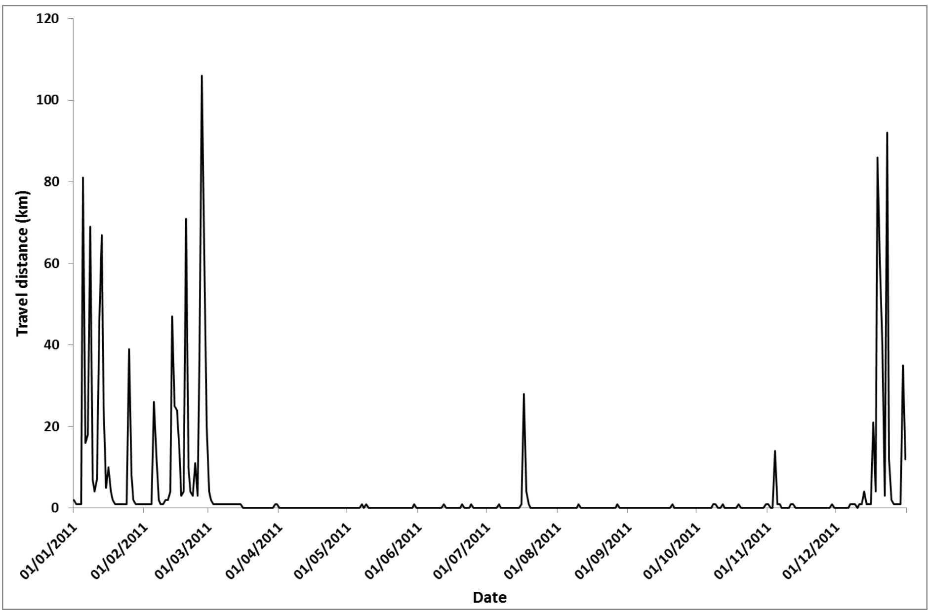
Figure 7. The distance from the source from which a particle has travelled to the catchment outlet for each day of 2011 for 80 µm particles.
