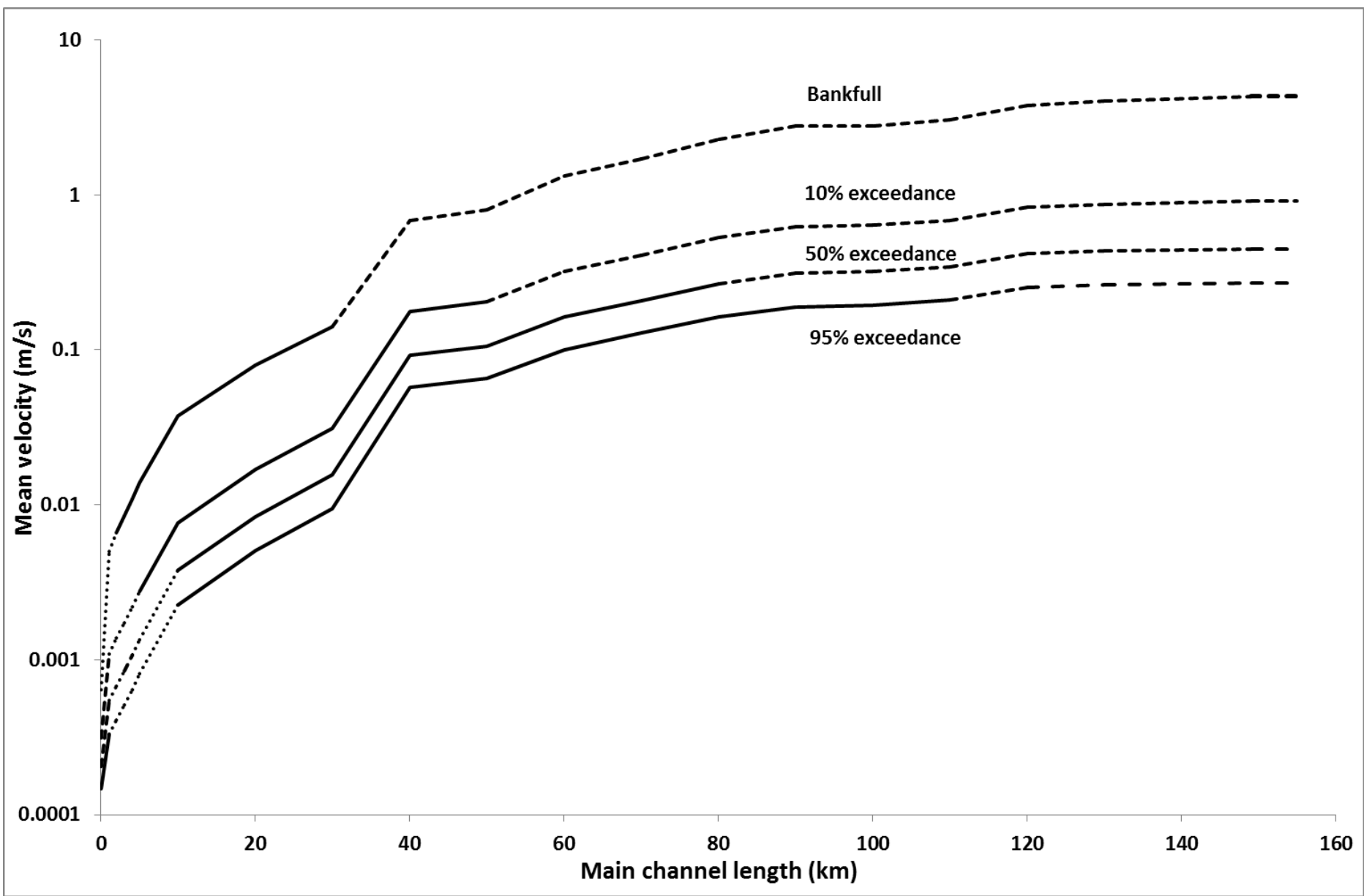
Figure 8. The classification from the Hjulstrom curve (... = deposition dominated; _ = transport dominated; and ---- = erosion dominated) for a range of velocity profiles for a 2 μm particle.
