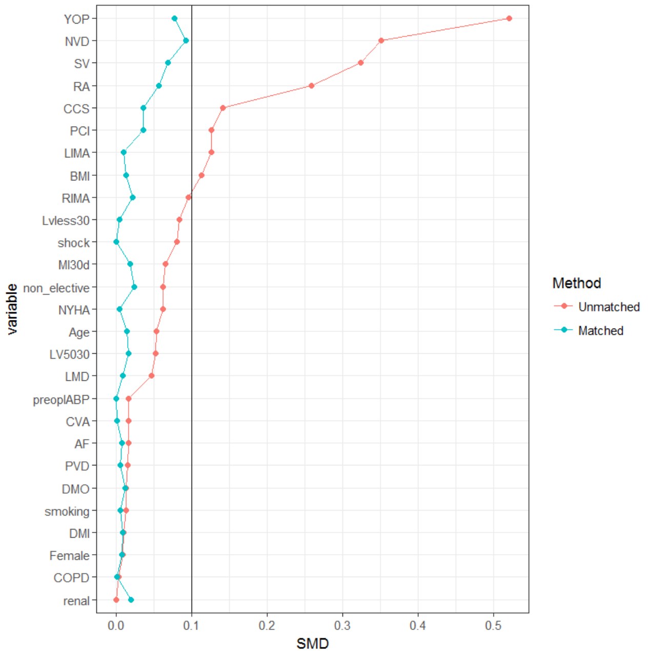
Figure 2: Changes in standardized mean difference (SMD) after matching for all variables included in the PS model.
