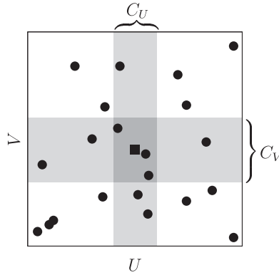
Figure 1: The calculation of I_{KL}(\mathcal{P}; h) . The U -space corresponds to the horizontal direction and the V -space to the vertical. Of course, this is a cartoon; these spaces are not one-dimensional, and they do not even have a defined dimension. The points in \mathcal{P} are marked as filled circles and a square; the square is the one whose contribution to I_{KL}(\mathcal{P}; h) is being calculated. The gray bars represent C_U(\blacksquare) and C_V(\blacksquare) with h = 7 ; that is, each of the gray rectangles contains seven points. \#C(\blacksquare) = 4 since it counts the points in the intersection, that is, the region with darker shading.
