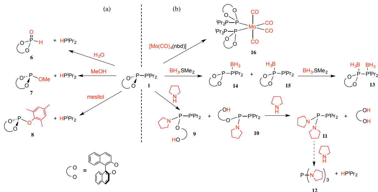
Scheme 2 Reactions undergone by phosphophosphidite 1 involving (a) P–P bond cleavage or (b) P–P bond retention
