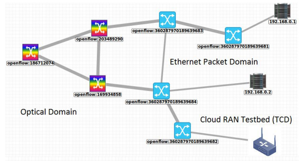
Fig. 3 University of Bristol testbed with the connection to TCD
