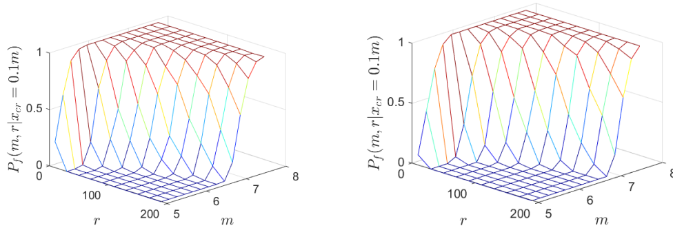
Figure 3. Fragility surface P_f(m, r) for x_{cr} = 0.1 m for the uncontrolled cable (left) and TID-controlled cable (right).
