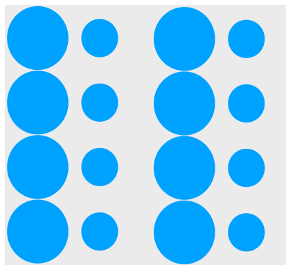
Figure 6. Schematic representation of a block of motifs measuring approximately 4 \times 4 \mu\text{m} . The vertical separation between motif centres is x = 1 \mu\text{m} while the horizontal separation is y = 2.1 \mu\text{m} .
