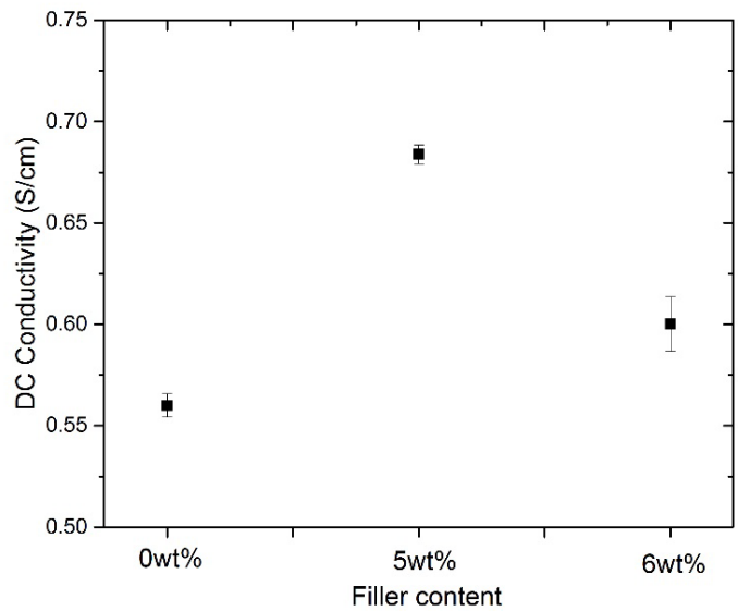
Figure 5: Transverse electrical conductivity versus filler content.
