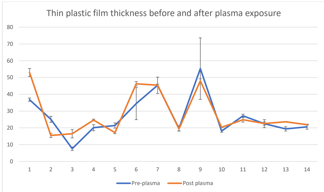
Fig.S1: Thin plastic film thickness before and after plasma exposure. X-axis represents the sample and y-axis represents the thickness in \mu\text{m}
