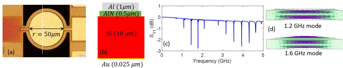
Fig. 1. (a) Optical microscope image of a representative device (b) Device cross-section showing the different layers and thicknesses (c) Measured RF S_{11} of a device showing the successive acoustic resonant modes in the device (d) Finite element simulation of the displacement profile of two of the modes supported by the cavity.
