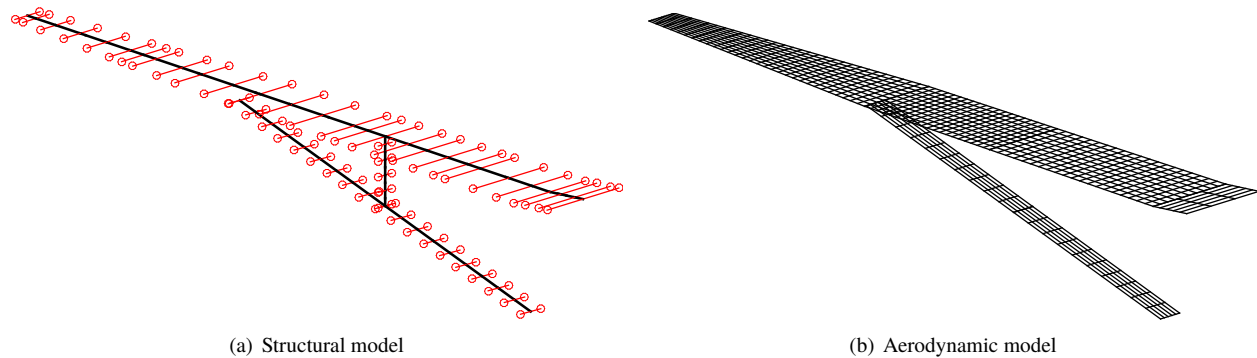
Fig. 4 Structural and aerodynamic model for the TBW
