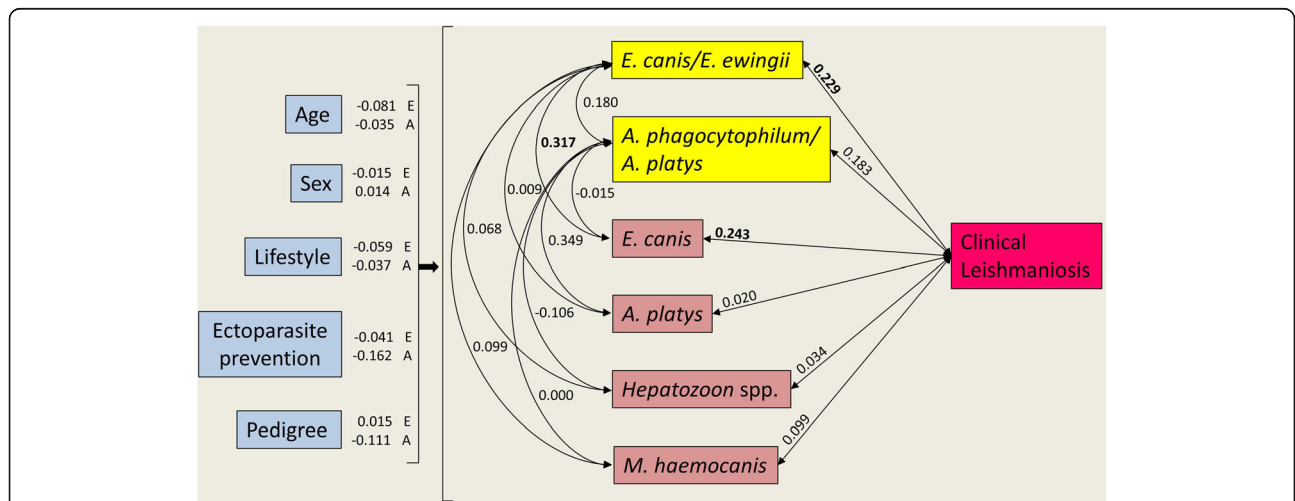
Fig. 2 Structural equation model showing predictors of vector-borne serological exposure status (except ClinL), and pathogen covariance (including ClinL), in domestic dogs. Values represent standardised coefficients among variables. Single headed arrows represent directional/causal relationships and double headed arrows covariance relationships among pathogens. For image clarity the serological status is in yellow boxes and the coefficients of host characteristics predicting pathogens are listed next to each host characteristic. The covariances E. canis , A. platys , Hepatozoon spp. and M. haemocanis were PCR-based diagnosed. In all cases, except age, variables are binomial (0 or 1) with 1 equal to male, outside, ectoparasitic prevention use, pedigree and positive pathogen status. Standardised coefficients with significant relationships of P \leq 0.05 (also see Table 2) are denoted in bold. Abbreviations: ClinL, clinical leishmaniosis; E. canis , Ehrlichia canis; E. ewingii , Ehrlichia ewingii; A. phagocytophilum , Anaplasma phagocytophilum; A. platys , Anaplasma platys; M. haemocanis , Mycoplasma haemocanis
