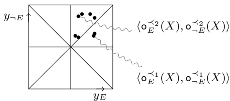
Figure 7: Plotting the \langle \circ_E^{\prec}(X), \circ_{\neg E}^{\prec}(X) \rangle corresponding to each \prec for example 7.
