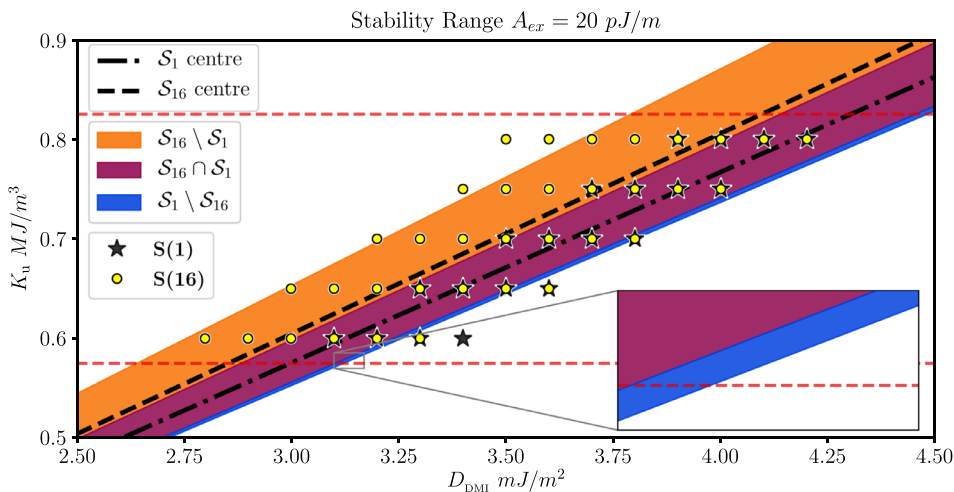
FIG. 2. Stability ranges for S(1) and S(16) bags. Plot for A_{\text{ex}} = 20 \text{ pJ m}^{-1} . We define the set \mathcal{S}_n = \{(D_{\text{DMI}}, K_u, A_{\text{ex}}) \in \mathbb{R}^3 \mid \text{Skyrmion bag of type } \mathcal{S}(n) \text{ is stable}\} ; in this plot, we approximate these sets by fixing the exchange constant A_{\text{ex}} and shading the areas corresponding to gradients within one \sigma of the critical gradient taken from Table II. The horizontal dashed lines represent the boundary of the simulations we have performed. The inset highlights that \mathcal{S}_1 \setminus \mathcal{S}_{16} is not empty for this approximation.
