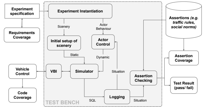
Fig. 2. Testbench Architecture.
