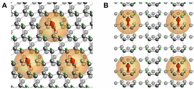
Fig. 5. Arrangements of impurity spins at the diamond surface for tight-binding calculations of YSR bands. (A) Triangular spin lattice for the (111) surface. (B) Rectangular spin lattice for the (100) surface. Green and black pellets represent the surface hydrogen and carbon atoms, respectively. Red arrows and orange spheres denote the impurity spins and localized YSR states, respectively. The hybridization of the localized YSR states gives rise to the emergence of YSR bands.
