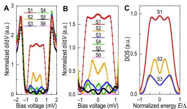
Fig. 4. Comparison between measured and calculated YSR bands. (A) Characteristic experimental spectra acquired at S1 to S6 in Fig. 2. The tunneling spectra are normalized to the conductance at 5 mV. (B) Magnification of the measured in-gap DOS. (C) YSR bands calculated using the tight-binding BdG equation in correspondence to the measured tunneling conductance spectra S1 to S3.
