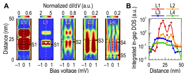
Fig. 3. YSR bands in hydrogenated boron-doped diamond. (A) Spatial and energy evolutions of the tunneling conductance, dI/dV , along the dashes in Fig. 2. The tunneling conductance along L1 is shown in two panels with different color scales for the clarity of both spatial and energy evolutions. Dash-dotted arrows (S1 to S5) indicate the location of the characteristic YSR bands as shown in Fig. 4A. (B) Spatial evolution of the integrated in-gap DOS. The integration was performed over the range from -1 to +1 mV. The solid curves are a guide to the eye.
