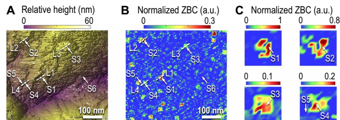
Fig. 2. Topography and spectroscopic mapping of zero-bias conductance in hydrogenated boron-doped diamond. (A) Topography of the diamond surface. Arrows (S1 to S6) indicate the location of the characteristic YSR bands as shown in Figs. 3A and 4A, and dashes (L1 to L4) indicate the direction of the spectroscopic mapping in Fig. 3A. (B) Zero-bias conductance map acquired at 0.5 K, well below the superconducting transition temperature. The map was constructed by normalizing the tunneling spectra to the dI/dV value at 5 mV, far outside the superconducting gap, and measuring the zero-bias conductance. The arrows and dashes indicate the same locations in (A), respectively. (C) Magnifications (39 nm \times 39 nm) of the “puddles” where the characteristic YSR bands in Figs. 3 and 4 are observed.
