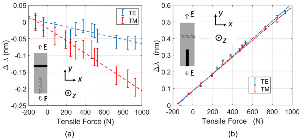
Fig. 8. The TE and TM response of the planar Bragg grating sensors in (a) the vertical and (b) the horizontal orientation with respect to the tensile load.
