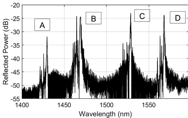
Fig. 7. Spectral back reflection of direct UV written Bragg gratings embedded into the planar chip.
