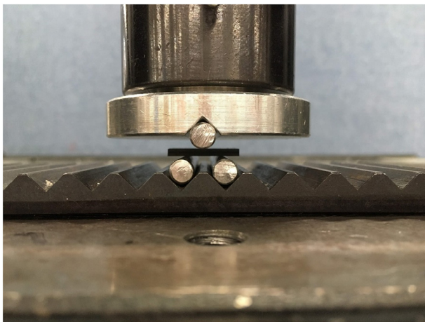
Fig. 3. Short beam shear test experimental arrangement.
