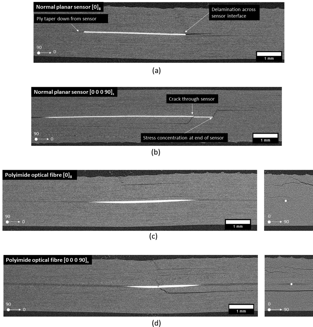
Fig. 4. X-ray CT cross-sections showing two modes of failure for the planar optical sensors (a) delamination across the sensor surface and (b) crack penetration through sensor, observed after short shear beam tests were conducted to failure. Comparison is made to failure modes of embedded optical fibre (c) [0]_8 layup and (d) [0\ 0\ 0\ 90]_s layup.
