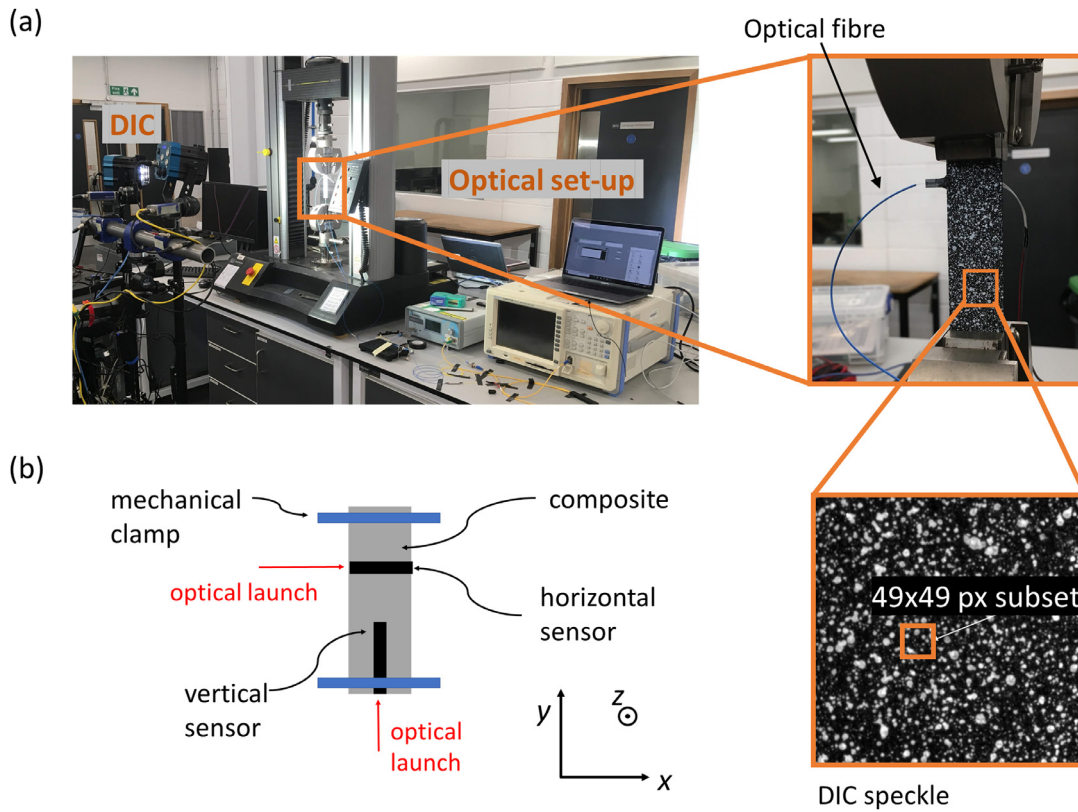
Fig. 6. Experimental arrangement for optical performance showing (a) photograph set-up and (b) schematic depicting the positioning of the optical planar sensors within the composite test piece. In this arrangement the loading direction is parallel to the y-axis.
