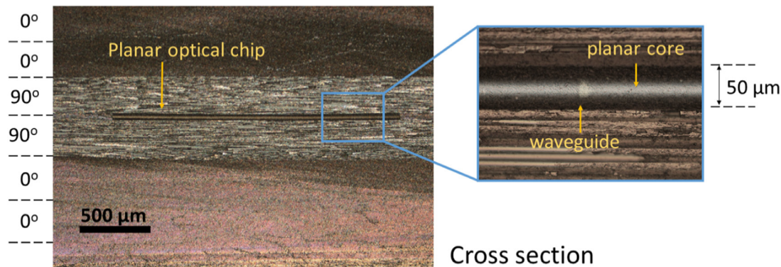
Fig. 2. Cross-sectional micrograph of an integrated optical chip embedded centrally in carbon fibre reinforced polymer [0/0/90] s . The planar silica chip is 50 μm thick and back illuminated with white light to observe waveguide and planar core layer.
