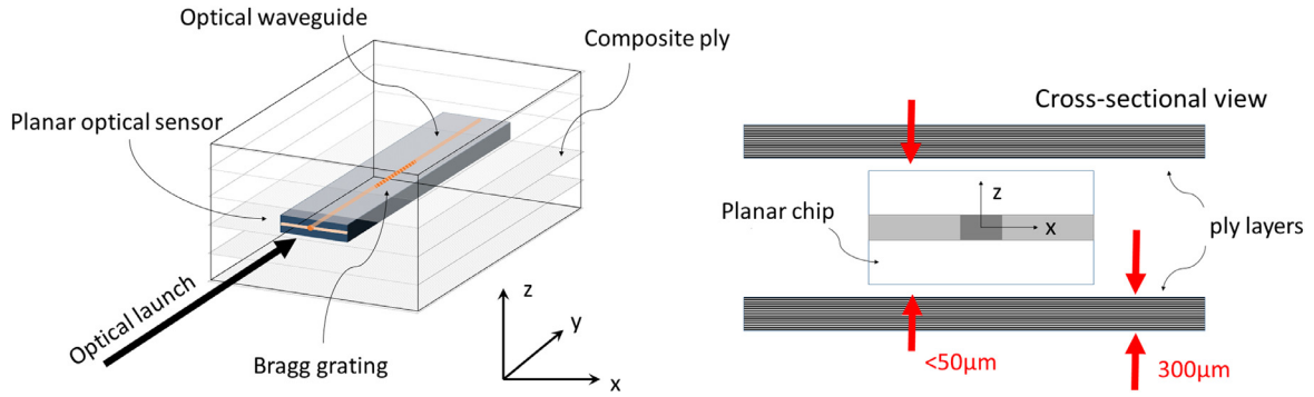
Fig. 1. A cross-sectional view of a planar waveguide (not to scale).
