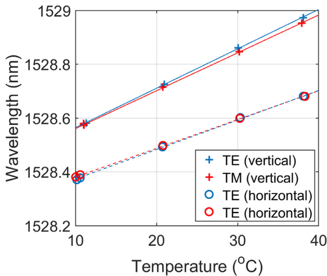
Fig. 9. Thermo-optic response of the TE and TM mode in horizontal and vertical orientation.
