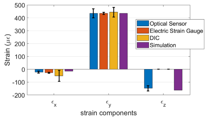
Fig. 10. A bar chart comparing the inferred strain response from the optical Bragg sensor compared to that measured through electrical strain gauge (in-plane components) through-thickness component using numerical simulations, for a 1 kN load along the y-dimension.
