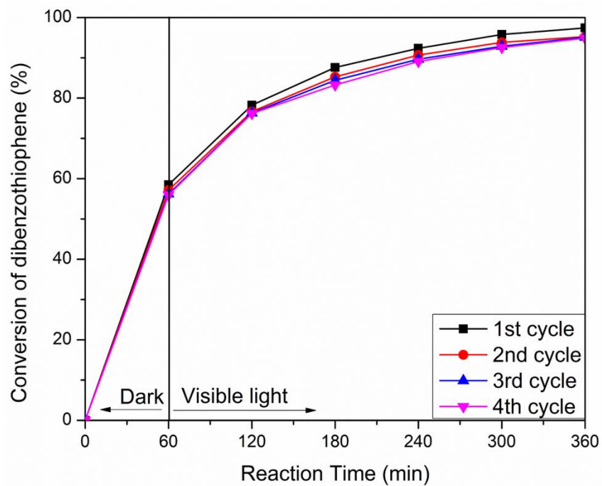
Fig 16. Photocatalytic degradation of DBT in successive cycles by 30% Ag@AgBr/Al-SBA-15.
