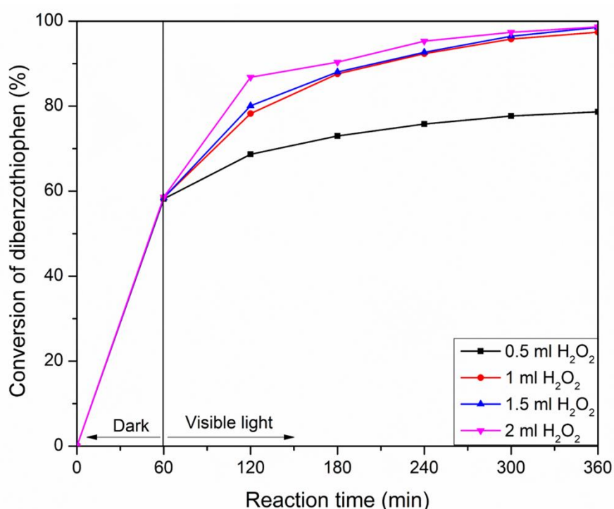
Fig 10. Photodegradation of DBT by 30% Ag@AgBr/Al-SBA-15 catalyst at different H 2 O 2 oxidant amounts under sunlight irradiation. (Reaction conditions: V model oil = 50 mL, m catalyst = 50 mg, reaction temperature = 70 °C)
