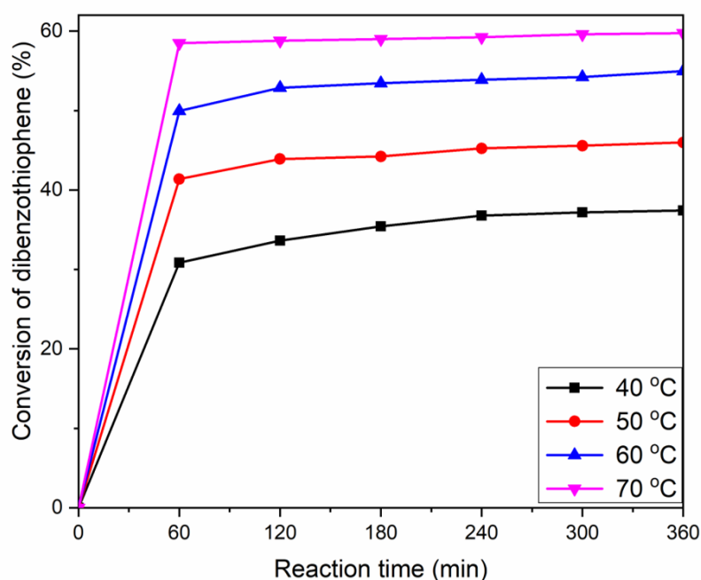
Fig 11. Effect of reaction temperature on photodegradation of DBT in the dark (Reaction conditions: V_{\text{model oil}}=50 mL, m_{\text{catalyst}}=50 mg, V_{\text{H}_2\text{O}_2}=1.0 mL)
