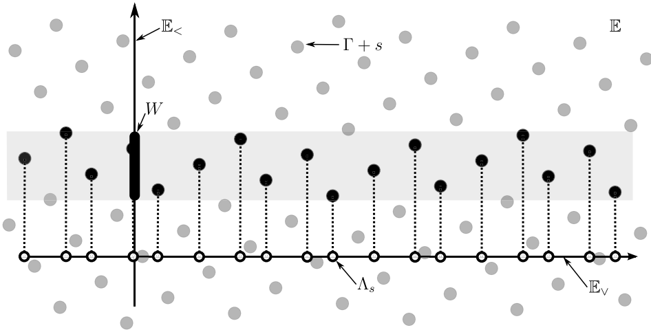
FIGURE 1. The definition of a cut and project set.
