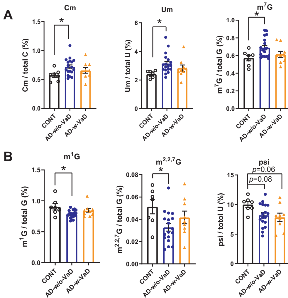
Fig. 4. Small RNA modifications in the 30–40-nt fraction from samples of the prefrontal lobe cortex of dementia patients with and without co-occurring vascular dementia patients. Changes in (A) 2'-O-methylcytidine (Cm), 2'-O-methyluridine (Um) and 7-methylguanosine ( m^7G ) modifications, and (B) 1-methylguanosine ( m^1G ), N^2,N^2 -dimethylguanosine ( m^{2,2,7}G ) and pseudouridine (psi or \Psi ) modifications in the cortex of AD-w/o-VaD, AD-w-VaD, and CONT subjects (each dot in the figure represents value from one independent sample); * P < 0.05 vs. CONT by Ordinary One-way ANOVA with post hoc Bonferroni correction.
