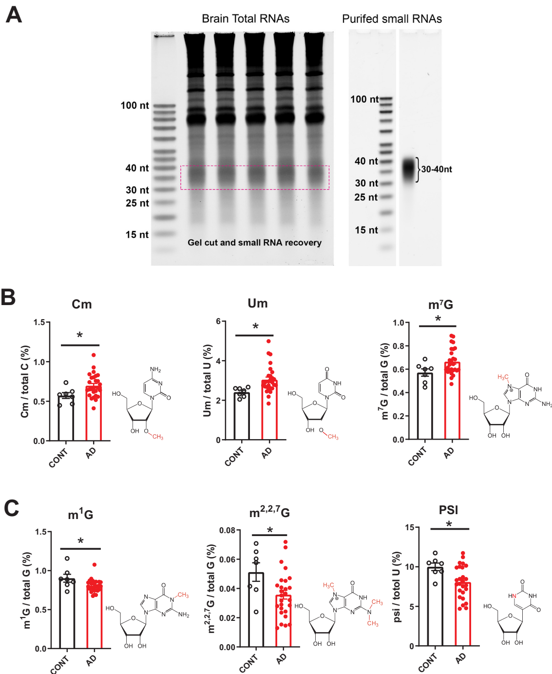
Fig. 3. Small RNA modifications in the 30–40-nt fraction from samples of the prefrontal lobe cortex of dementia patients. (A) Representative image showing purification of 30–40-nt small RNAs for the analysis of RNA modifications. (B) Increases in 2'-O-methylcytidine (Cm), 2'-O-methyluridine (Um) and 7-methylguanosine ( m^7G ) modifications, and (C) reductions in 1-methylguanosine ( m^1G ), N^2,N^2 -dimethylguanosine ( m^{2,2,7}G ) and pseudouridine (psi or \Psi ) modifications in the cortex of AD compared with CONT subjects (each dot in the figure represents value from one independent sample); * P < 0.05 vs. CONT by Student t -test.
