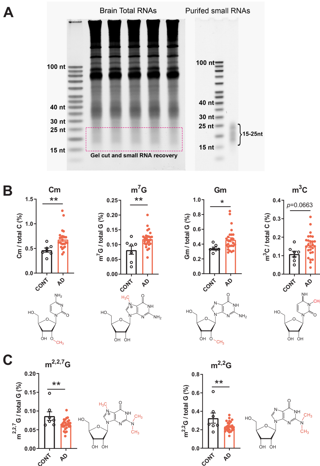
Fig. 1. Small RNA modifications in the 15–25-nt fraction from samples of the prefrontal lobe cortex of dementia patients. (A) Representative image showing purification of 15–25-nt small RNAs for the analysis of RNA modifications. (B) Increases in 2'-O-methylcytidine (Cm) 7-methylguanosine (m 7 G), 2'-O-methylguanosine (Gm), and 3-Methylcytidine(m 3 C) modifications. (C) Reductions in N 2 ,N 2 ,7-trimethylguanosine (m 2,2,7 G) and N 2 ,N 2 -dimethylguanosine (m 2,2 G) modifications in the cortex of AD compared with CONT subjects (each dot in the figure represents value from one independent sample); *P < 0.05;**P < 0.01 vs. CONT by Student t-test.
