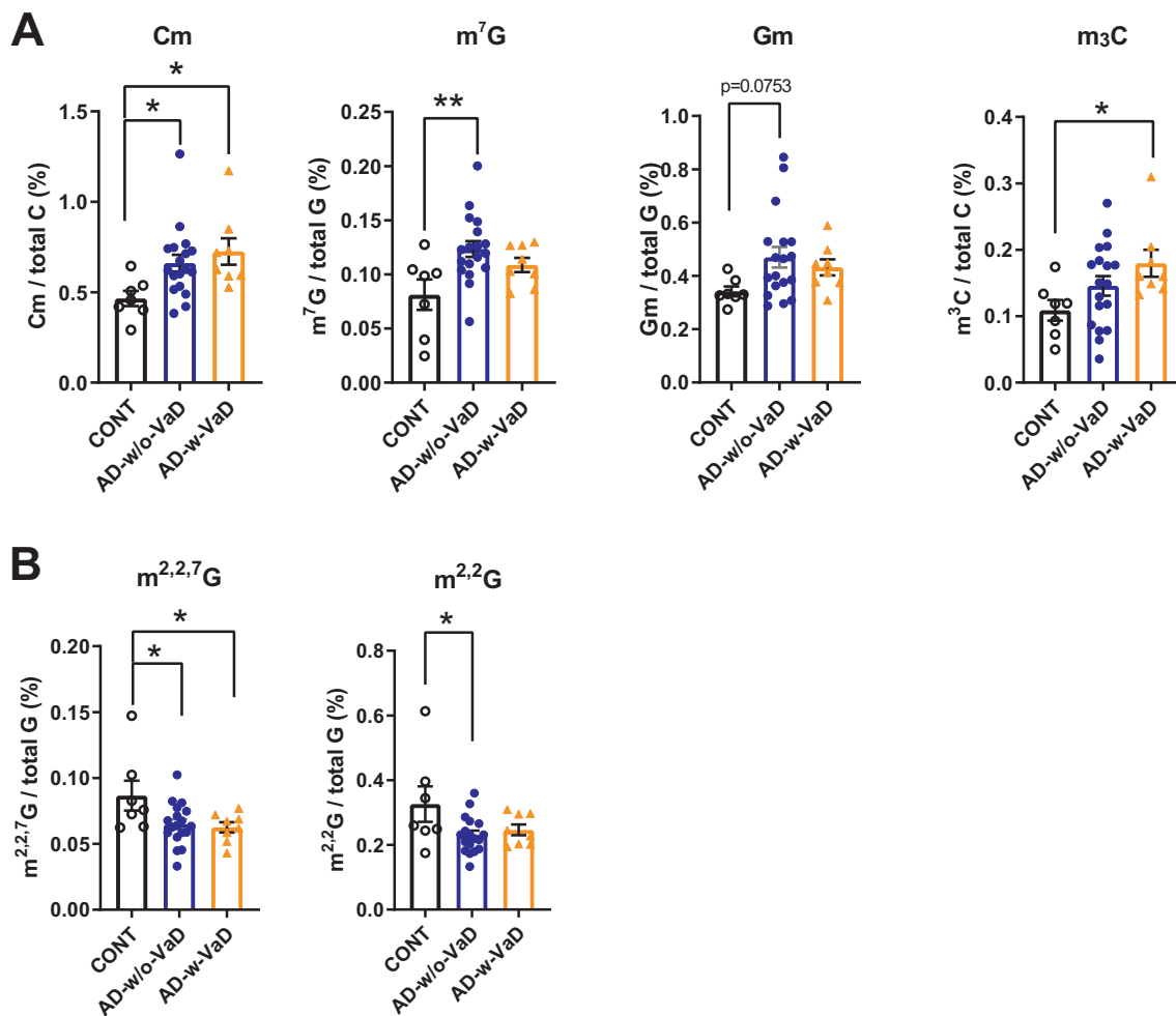
Fig. 2. Small RNA modifications in the 15–25-nt fraction from samples of the prefrontal lobe cortex of dementia patients with and without co-occurring vascular dementia patients. (A) Increases in 2'-O-methylcytidine (Cm) 7-methylguanosine ( m^7G ), 2'-O-methylguanosine (Gm), and 3-Methylcytidine ( m^3C ) modifications. (B) Reductions in N^2,N^2,7 -trimethylguanosine ( m^{2,2,7}G ) and N^2,N^2 -dimethylguanosine ( m^{2,2}G ) modifications in the cortex of AD-w/o-VaD, AD-w-VaD, and CONT subjects (each dot in the figure represents value from one independent sample); * P < 0.05 ; ** P < 0.01 vs. CONT by Ordinary One-way ANOVA with post hoc Bonferroni correction.
