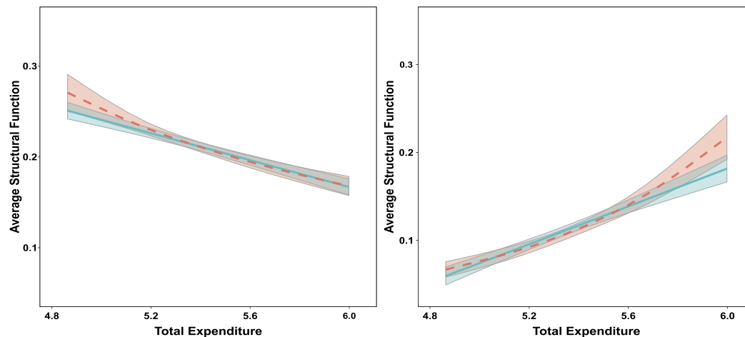
FIGURE 2. ASF for food (left) and leisure (right). Quantile (solid) and distribution regression (dashed).
