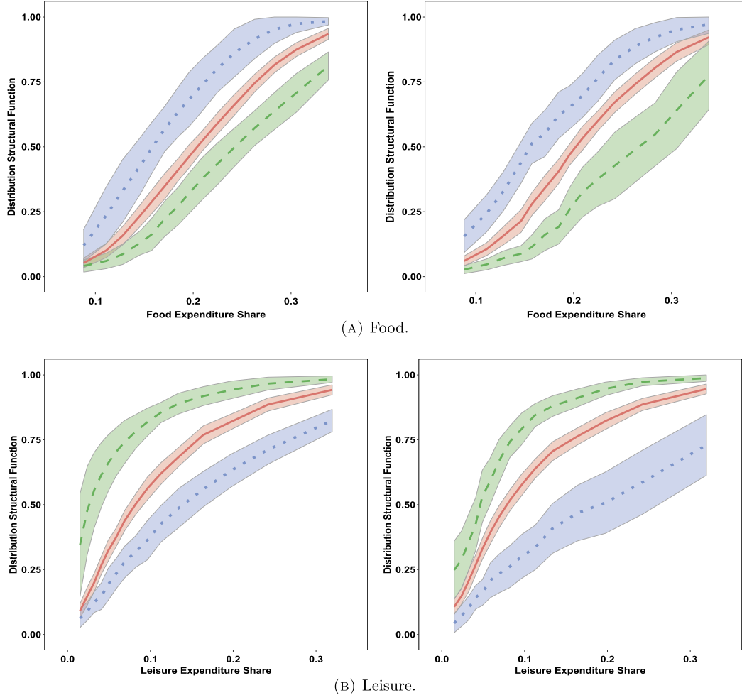
FIGURE 3. DSF. DSF at X = \widehat{Q}_X(0.1) (dashed), X = \widehat{Q}_X(0.5) (solid), X = \widehat{Q}_X(0.9) (dotted). Quantile (left) and distribution regression (right).
