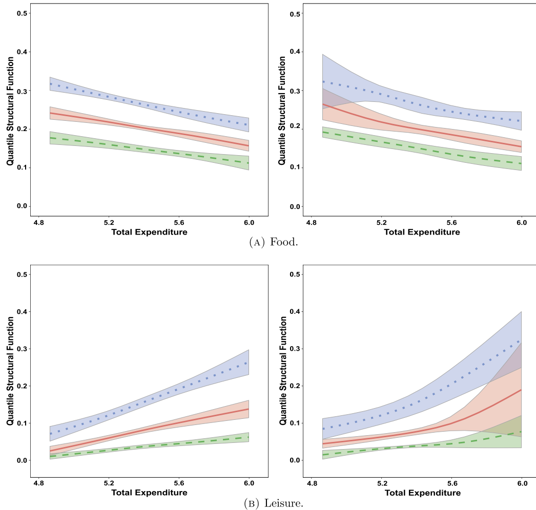
FIGURE 1. QSF 0.25-QSF (dashed), 0.5-QSF (solid), and 0.75-QSF (dotted). Quantile (left) and distribution regression (right).
