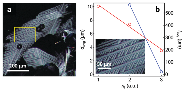
Fig. 7 (a) PLM image of the feather-like aggregates in 1.2 wt% SDS-in-glycine gel, with the rectangular region showing where tertiary fibres were measured. (b) Average lengths, l_{\text{avg}} (blue circles), and diameters, d_{\text{avg}} (red circles), of fibres vs. the fibre order, n_f . (inset) The highlighted region in (a) magnified for clarity.
